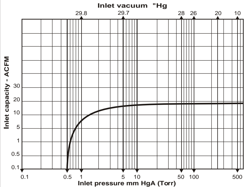
Performance curve: RVL020H
